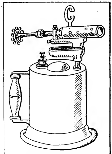
Fig. 4—Gasoline torch for soldering
